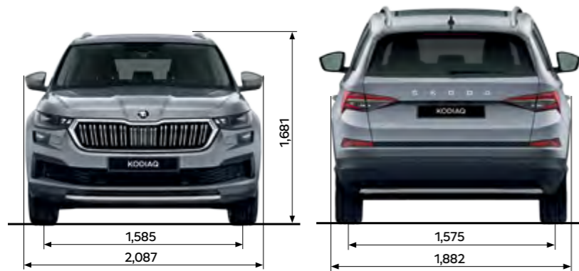
Dimensions (5-seat)
